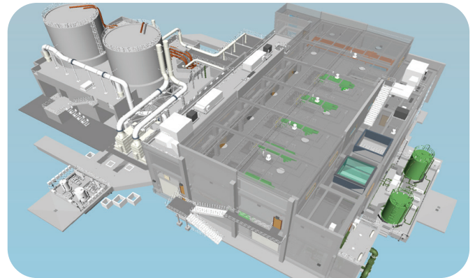
Possible concept for a new mechanical dewatering facility
